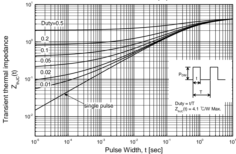
TMPF4N60AZ(G)
