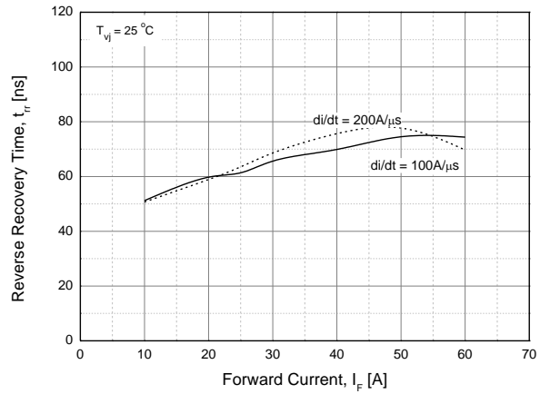
Fig. 22 Reverse Recovery Time vs. Forward Current
