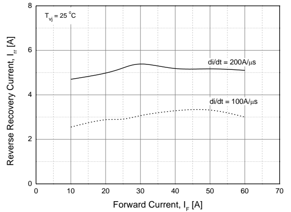
Fig. 20 Reverse Recovery Current vs. Forward Current
