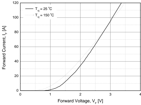
Fig. 19 Diode Conduction Characteristics
