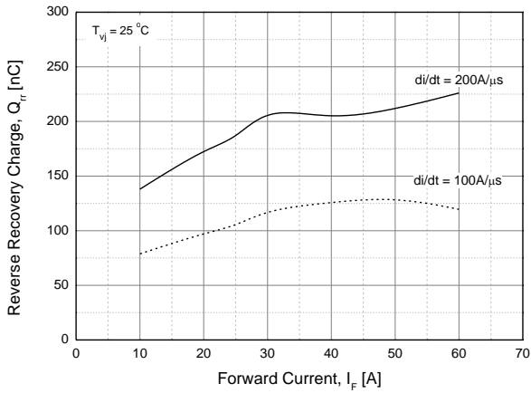
Fig. 21 Reverse Recovery Charge vs. Forward Current
